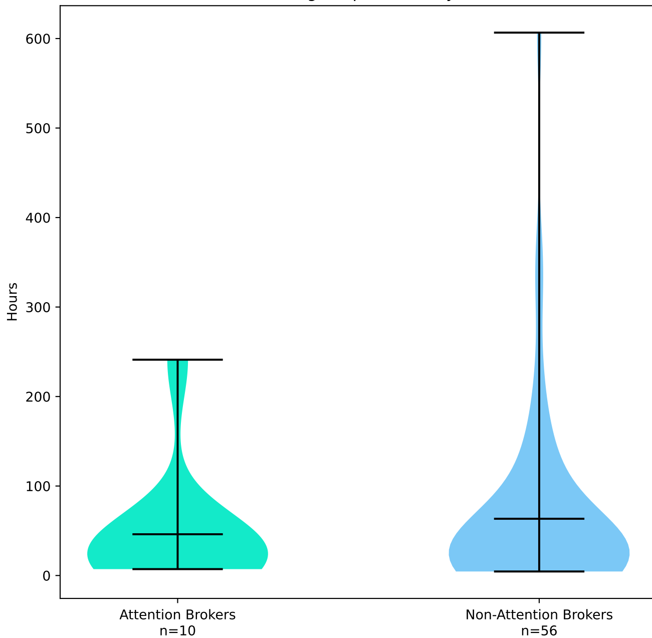
Average Repost Latency
